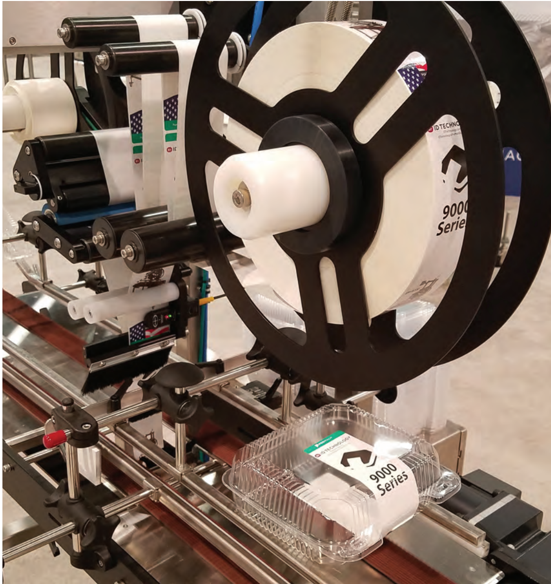
EPI 9220 applying a C-Wrap label to a clamshell container
