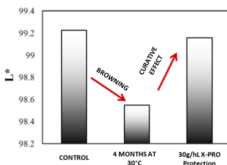
FIGURE 8. CURATIVE ACTION OF X-PRO® PROTECTION. Laboratory tests were performed by measuring the CIELAB analysis of color of a white wine before and after 4 months of storage at 30°C. The healing effect of X-PRO® PROTECTION is evidenced by the decrease in yellow ( b^* ) and the increase in brightness ( L^* ) following a dosage of 30 g/hL.
