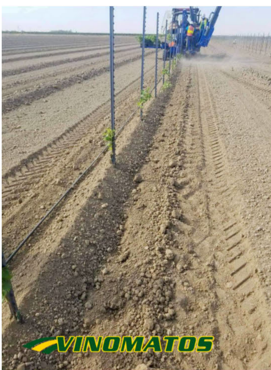
Vineyard planting service in Arbutle – USA with Révolution planting machine
