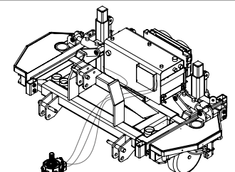
With direct pump (to the rear PTO)
