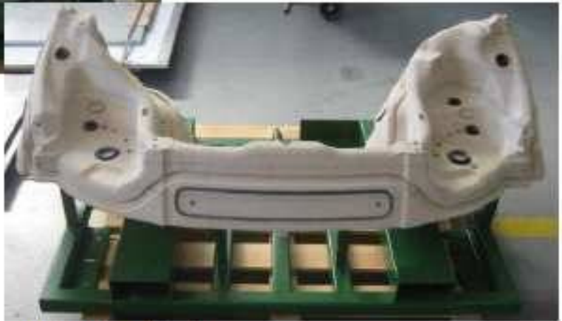
Trimming Fixture
