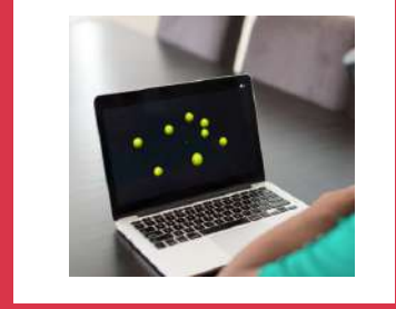
Perceptual-cognitive software
